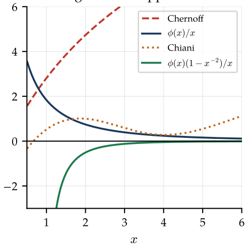
How tight is each approximation?
