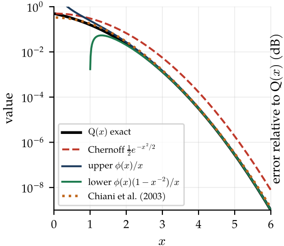
The Gaussian tail and its bounds
