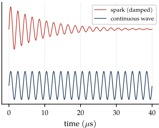
Waveforms
