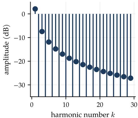
Odd harmonics fall as 1/k (-6 dB/octave)
