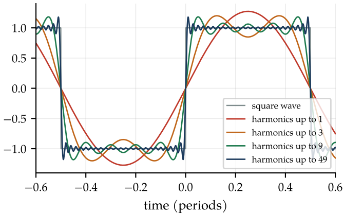
Partial Fourier sums and the Gibbs overshoot
