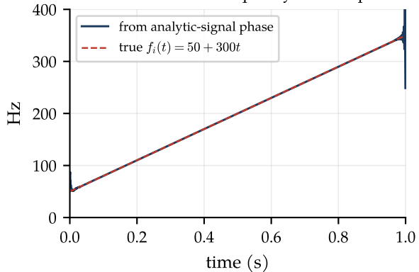
Instantaneous frequency of a chirp
