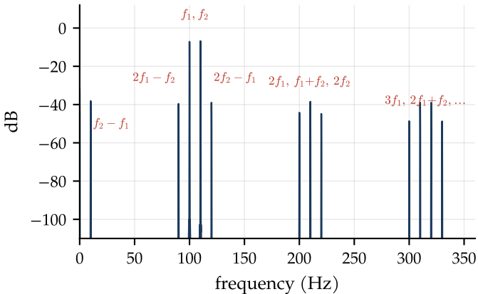
Two tones through y = a_1x + a_2x^2 + a_3x^3
