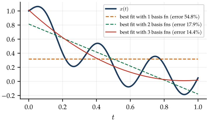
Projection onto Legendre polynomials
