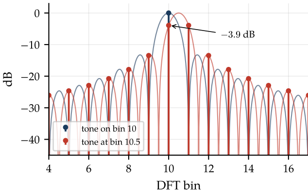
Rectangular window: the picket fence
