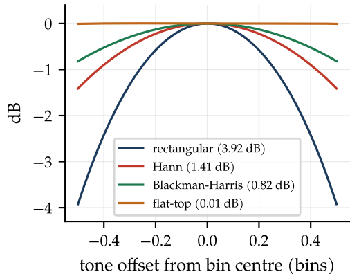
Scalloping loss
