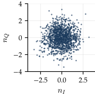
I/Q scatter: circular, corr = +0.036
