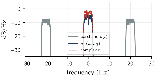
power spectral densities
