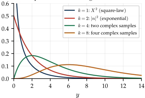
chi-square densities, k degrees of freedom
