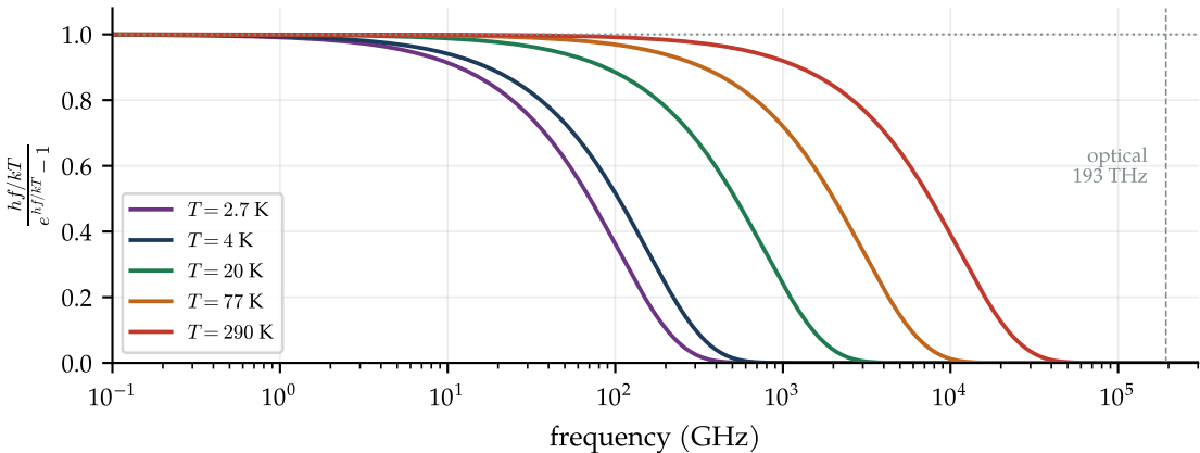
Thermal noise per hertz relative to the classical kT
