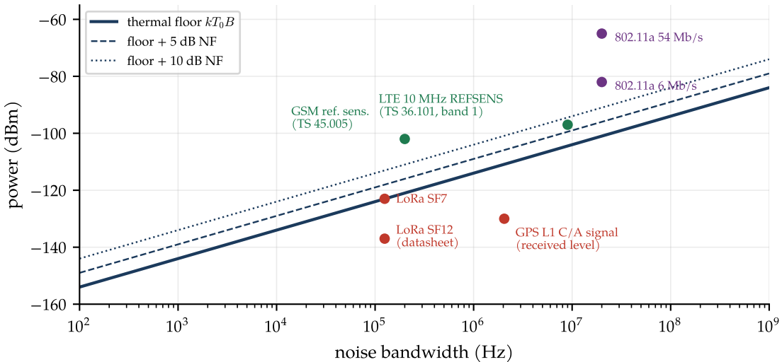
Thermal floor versus sensitivity of real receivers
