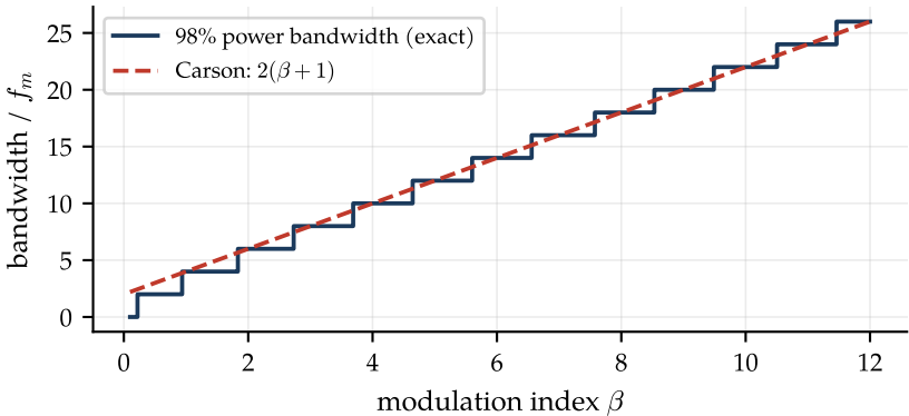
Carson's rule versus the true FM bandwidth
