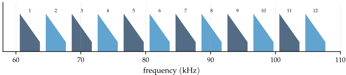
Basic group: 12 voice channels, lower sidebands of carriers 64, 68, ..., 108 kHz (60-108 kHz)
