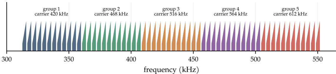
Basic supergroup: five groups translated to 312-552 kHz (60 channels)
