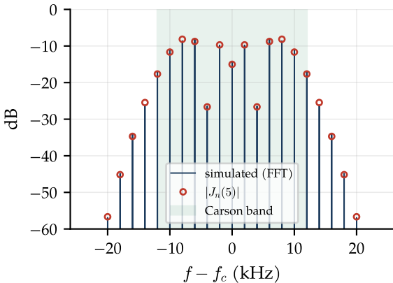
Tone FM, \beta = 5 , f_m = 2 kHz
