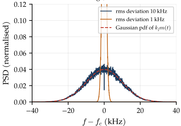
Gaussian message, 1 kHz bandwidth
