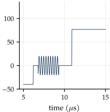
Zoom: sync, 9-cycle burst, first bars
