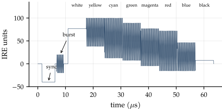
One line of NTSC colour bars (75%), 63.56 \mu\text{s}
