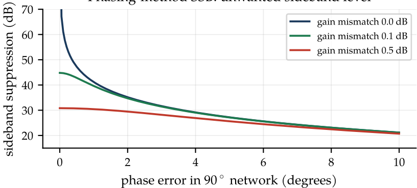
Phasing-method SSB: unwanted sideband level
