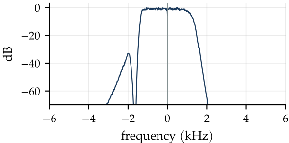
(c) after the two low-pass filters
