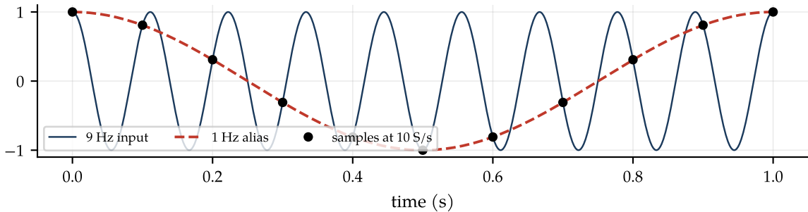
Two sinusoids that the sampler cannot tell apart
