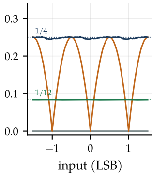
variance of error ( \text{LSB}^2 )
