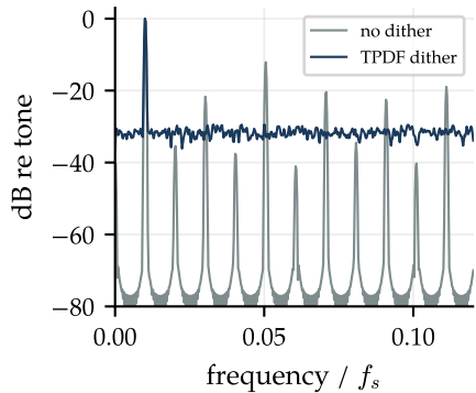
0.9-LSB sine: harmonics vs noise
