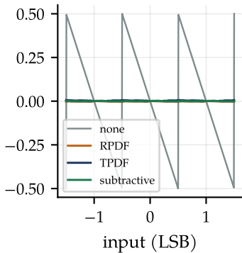
mean of error
