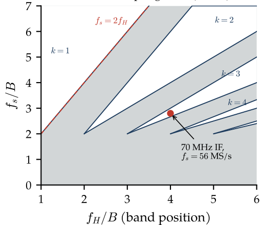
Allowed sampling rates (white)
