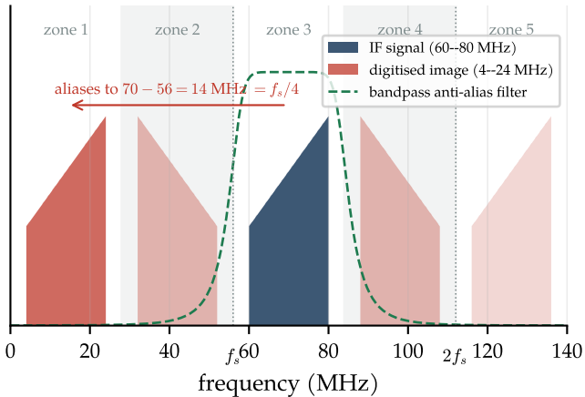
70 MHz IF sampled at f_s = 56 MS/s (third Nyquist zone)
