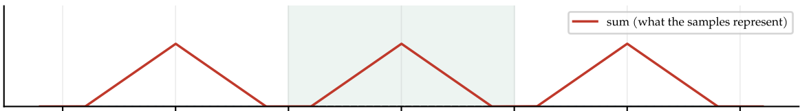
sampled at f_s = 2.5W : replicas separate
