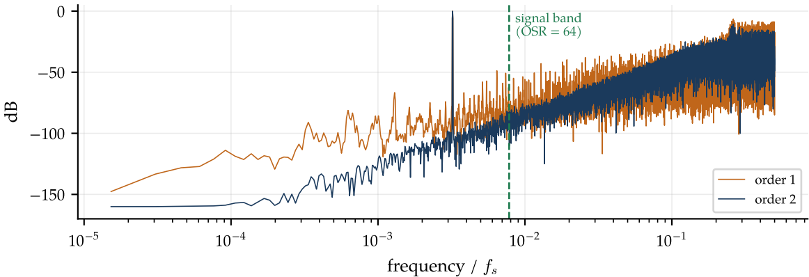
One-bit sigma-delta modulators push quantization noise out of band
