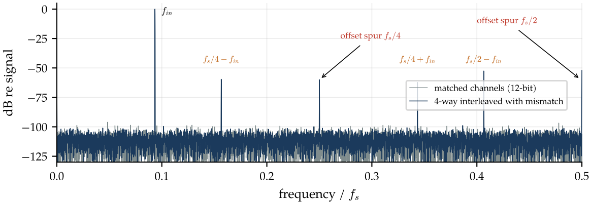
Interleaving spurs from 0.2--0.4% gain, 0.1--0.2% offset and 0.1--0.2% timing mismatch
