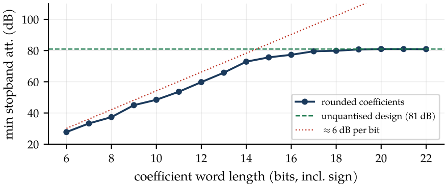
95-tap equiripple FIR: coefficient quantisation
