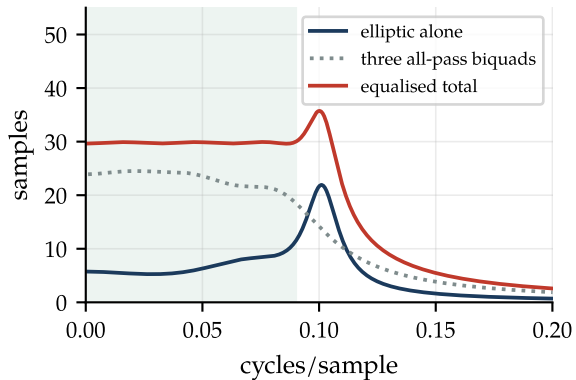
group delay (equalised band shaded)
