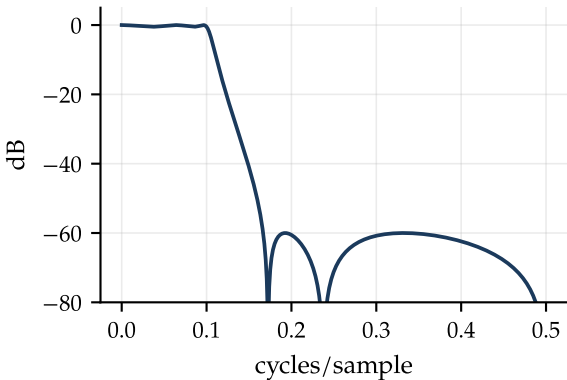
5th-order elliptic (all-pass leaves this unchanged)
