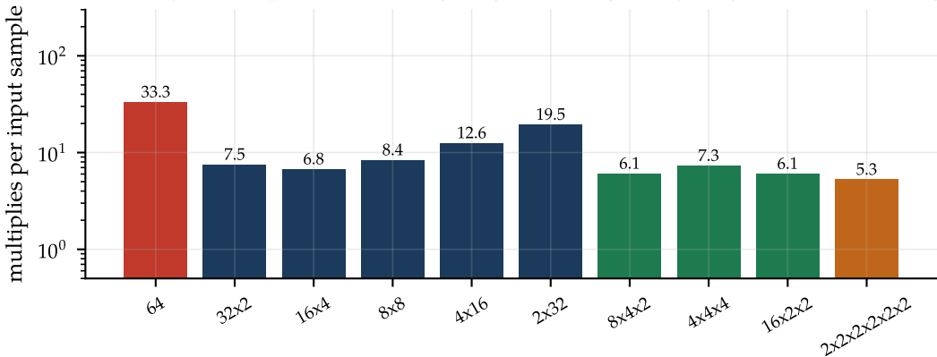
Decimation by 64, 80 dB, passband 0.4f_{out} : single stage (red), 2 stages (navy), 3 (green), half-bands (orange)
