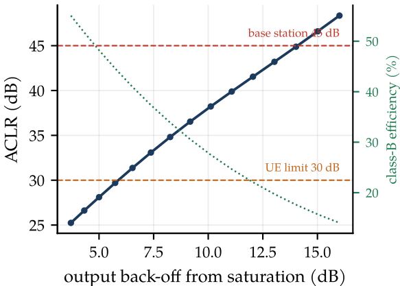
ACLR of 64-QAM OFDM through a PA
