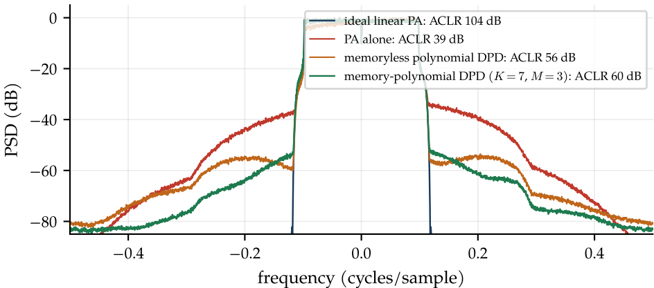
Digital predistortion of a PA with memory, 11 dB input back-off
