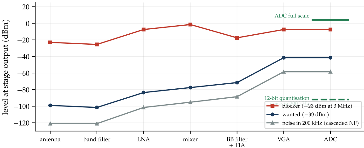
Level diagram: the wanted signal, the noise and a blocker through the chain
