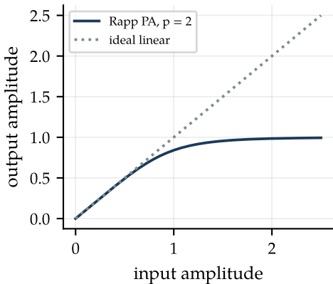
AM/AM characteristic
