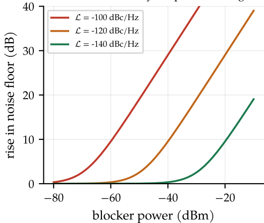
desensitisation by reciprocal mixing
