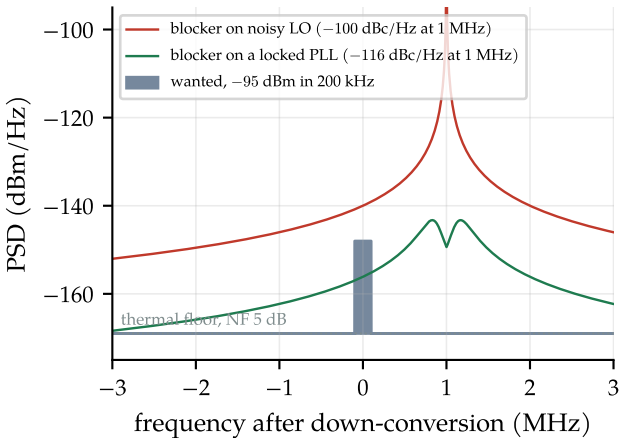
−40 dBm blocker 1 MHz away
