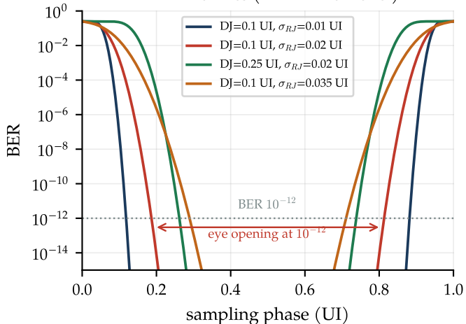
Bathtub curves (dual-Dirac model)
