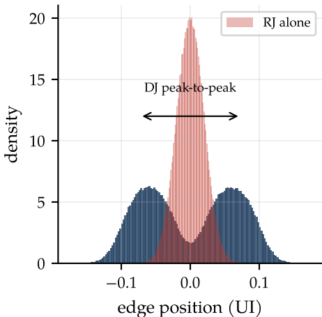
Total jitter histogram
