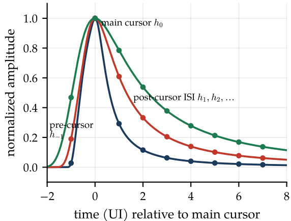
Single-bit (pulse) response
