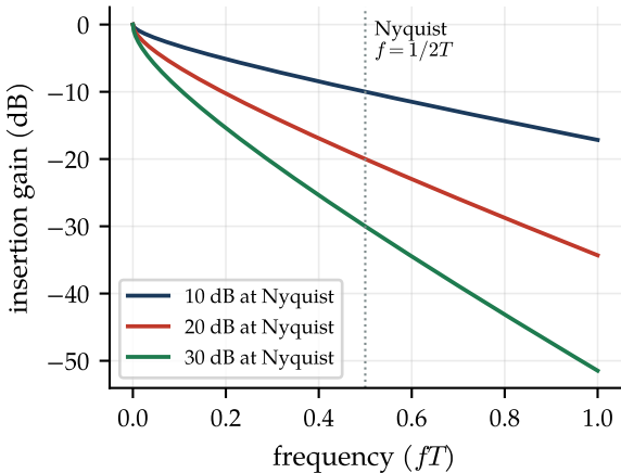
Channel loss (skin + dielectric)
