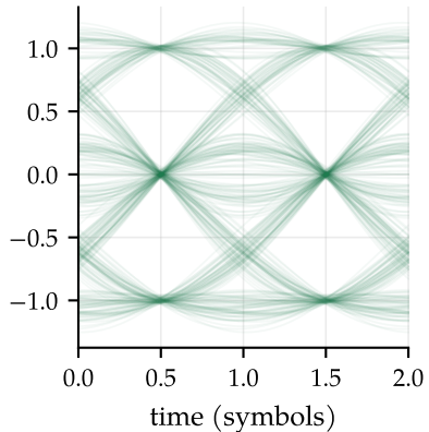
Duobinary eye: 3 levels
