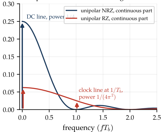
Unipolar codes: nonzero mean gives lines
