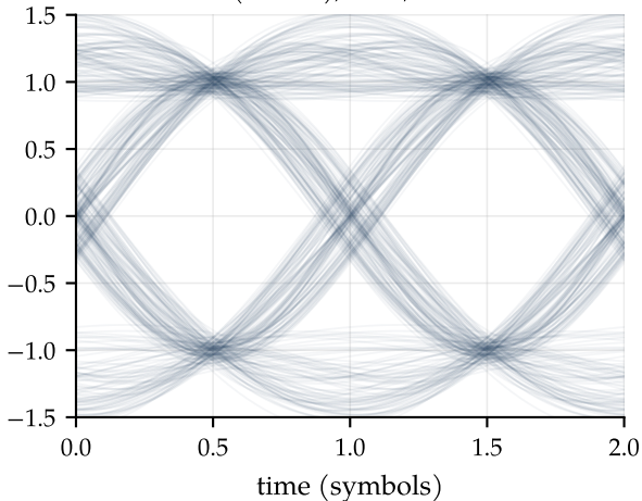
NRZ (PAM-2), 2 Gb/s at 2 GBd
