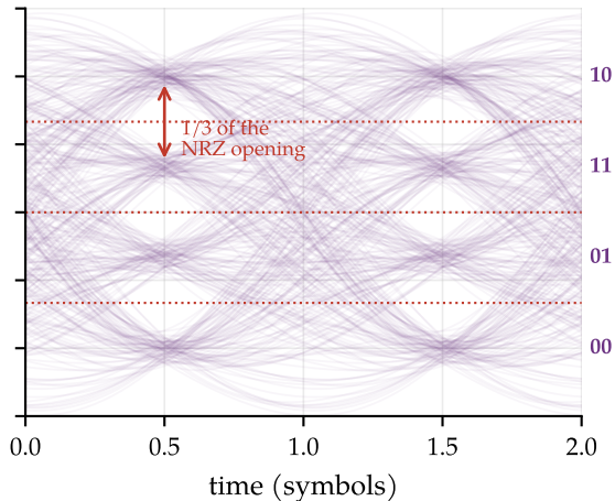
PAM-4, 2 Gb/s at 1 GBd (same peak swing)
