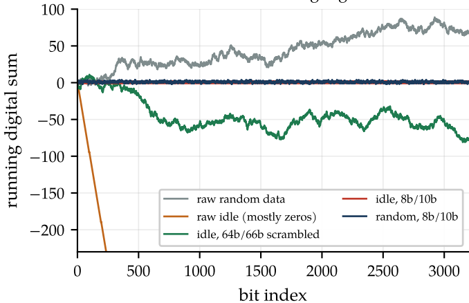
DC balance: the running digital sum
