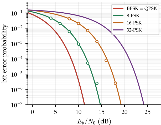
M -PSK (lines: exact / Gray approx.; markers: simulated)
