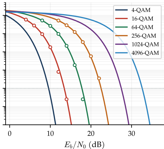
square M -QAM (Gray)
