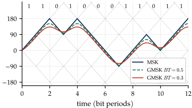
phase trajectory: MSK moves \pm 90^\circ per bit
