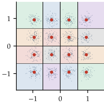
16-QAM: square cells
