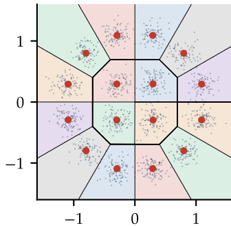
16-APSK: wedges and a ring
