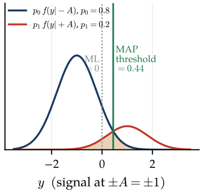
unequal priors move the boundary
