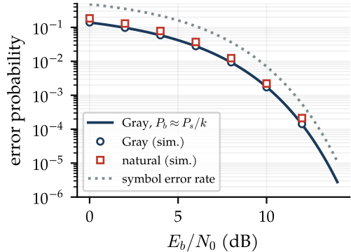
16-QAM bit error rate
