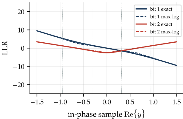
16-QAM in-phase bits, E_s/N_0 = 5 dB
