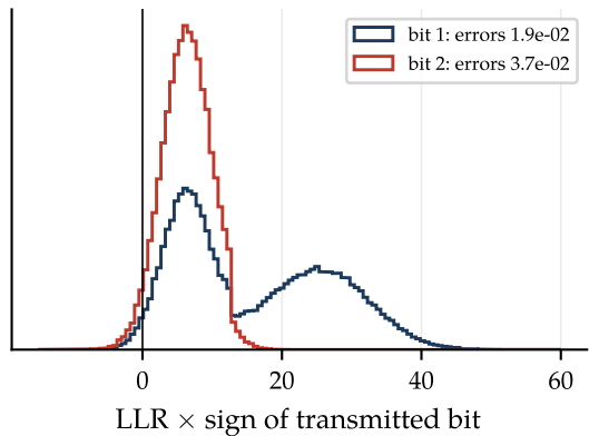
bit reliability, E_s/N_0 = 12 dB
