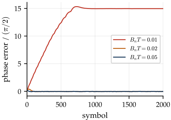
(a) pull-in of a QPSK DD loop, \nu = 0.008
