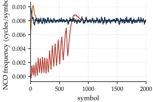
(b) NCO frequency (25-symbol average)
