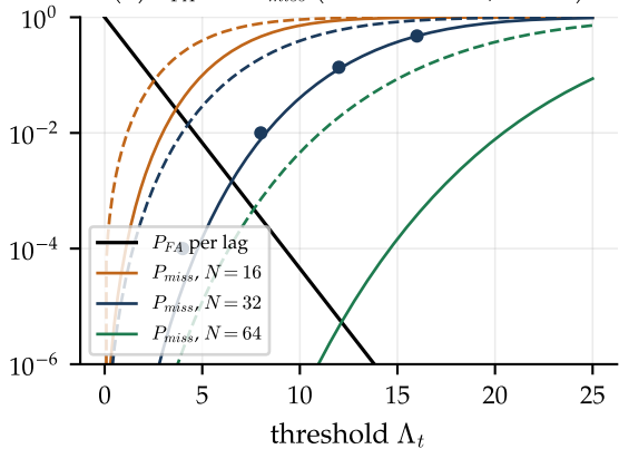
(b) P_{FA} and P_{miss} (dashed: -3 dB; o: sim.)
