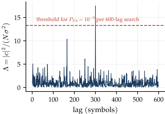
(a) 32-symbol preamble at E_s/N_0 = 0 dB
