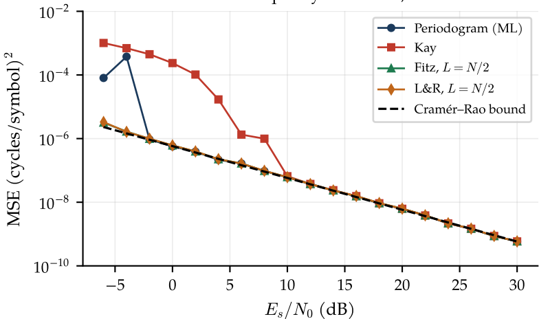
Data-aided frequency estimation, N = 64
