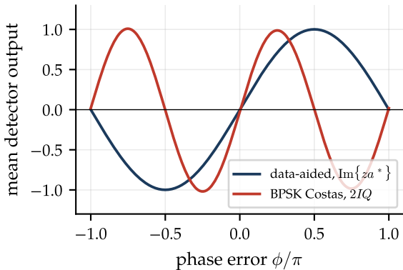
(a) data-aided and BPSK Costas, 10 dB
