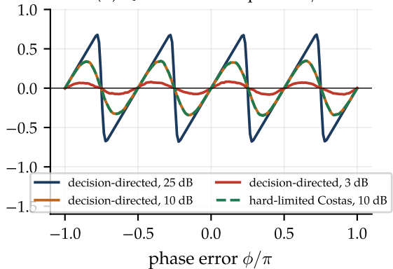
(b) QPSK detectors: period \pi/2
