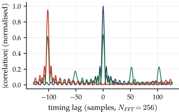
(a) LTE PSS (Zadoff-Chu, u = 25 )
