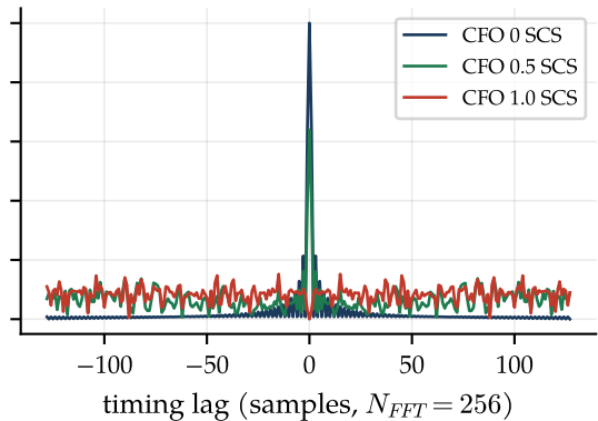
(b) NR PSS (m-sequence, 127)
