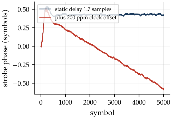
(a) Gardner loop, B_n T = 0.01 , E_s/N_0 = 20 dB
