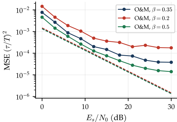
(b) Oerder--Meyr, L_0 = 100 (dashed: MCRB)
