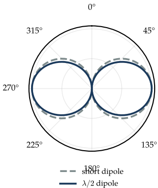
(a) dipole, E-plane
