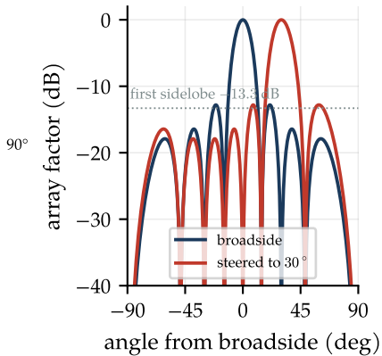
(b) 8-element array
