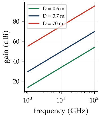
(c) dish, \eta = 0.6
