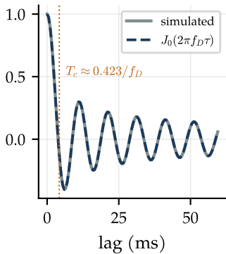
(b) autocorrelation
